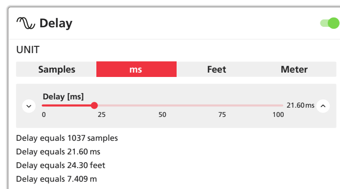
Fig. 25 View “Output – Delay”
