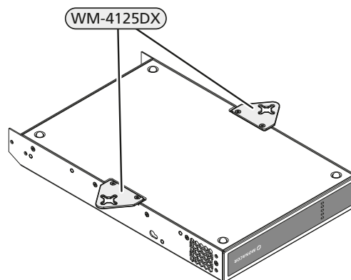
Fig. 8 Mounting plates on lower side of the device
