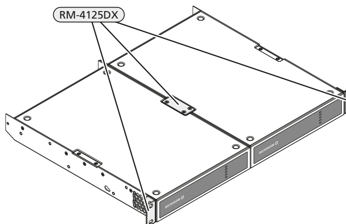
Fig. 7 Connecting plate and rack mounting brackets
