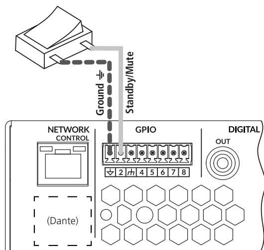
Fig. 11 external standby/mute switch
