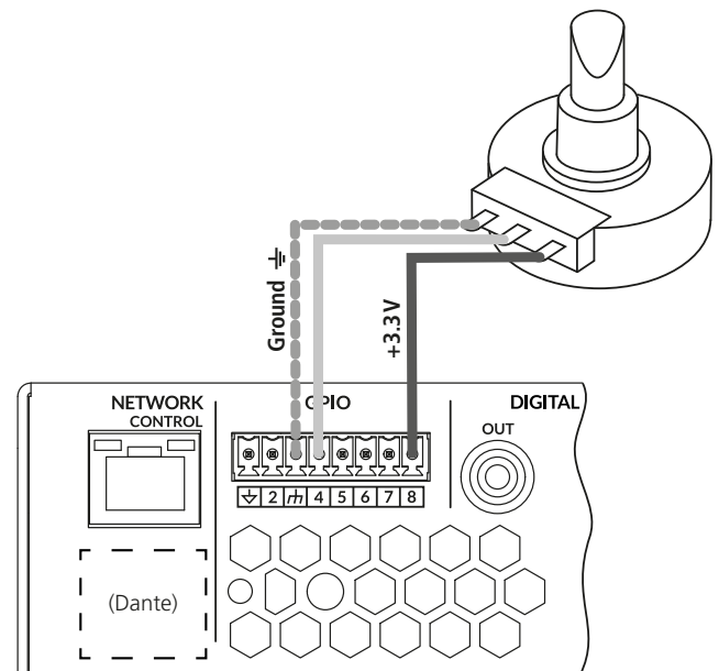
Fig. 10 external volume control
