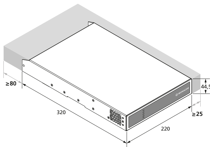
Fig. 4 Ventilation distances
