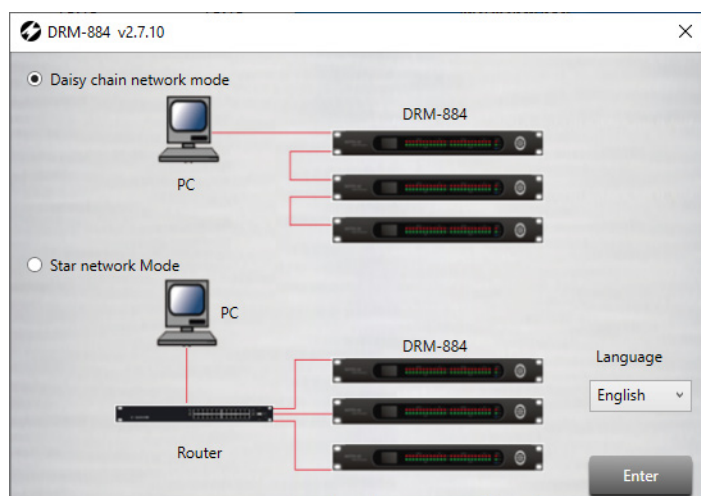
Fig. 13 Start window
