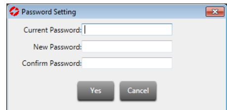
Fig. 30 Password Setting
