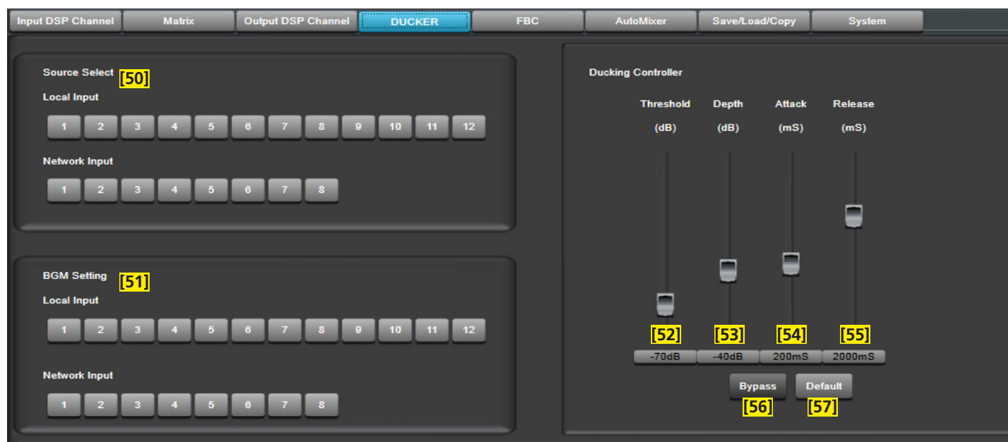
Fig. 23 View "Ducker"
