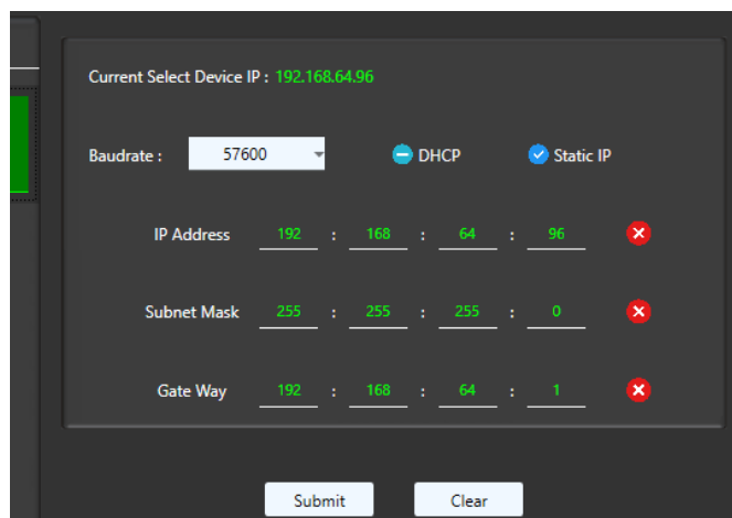
Fig. 19 Network details
