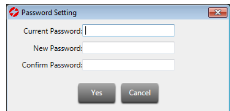
Abb. 30 Password Setting
