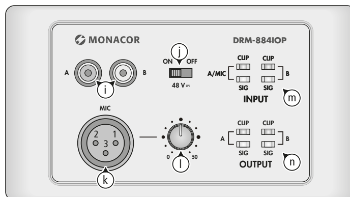
Fig. 36 DRM-884IOP
