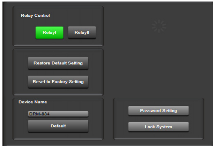
Fig. 29 View "System"
