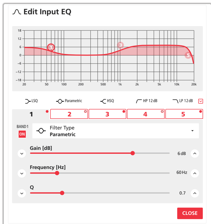
Fig. 11 Window "Input - Analog - Edit Input EQ"
