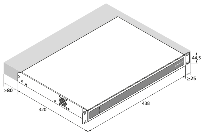
Fig. 4 Ventilation distances
