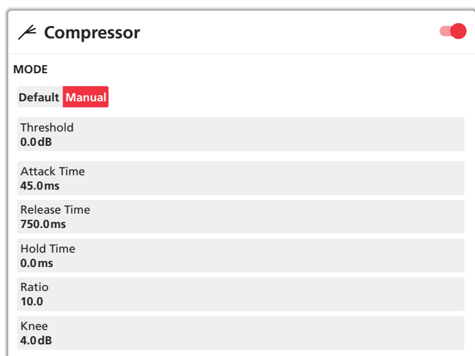
Fig. 17 View "Zone – Compressor"
