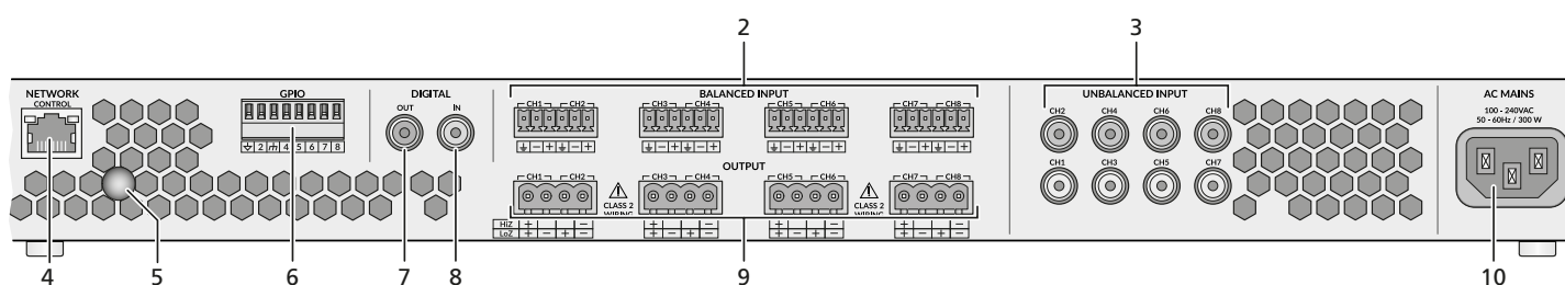
Fig. 3 Rear panel
