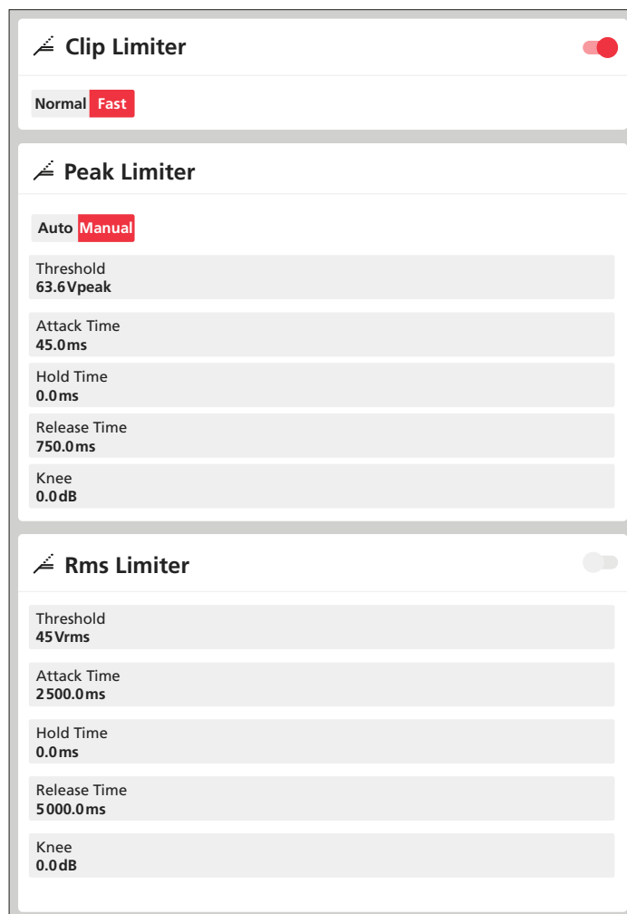
Fig. 26 View “Output – Speaker Preset – Limiter”
