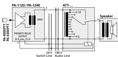
⑥ Emergency priority relays
