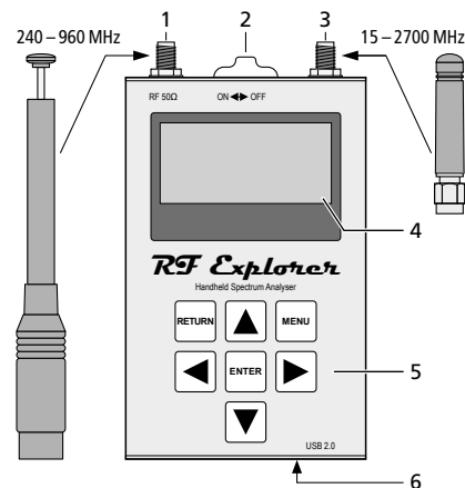
Fig. 1 Connections and operating elements
