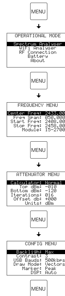
Fig. 4 Menu structure
