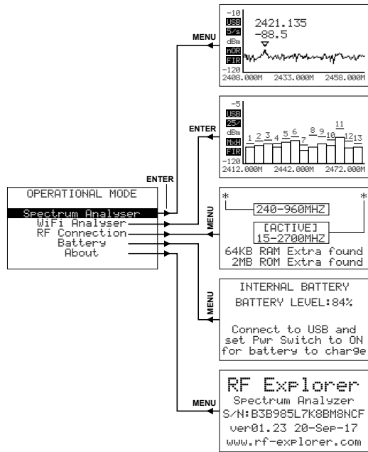
Abb. 5 Menü Operational Mode
